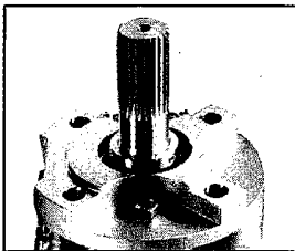
Rotor with Splines Hardened spline for positive coupling and long service.
